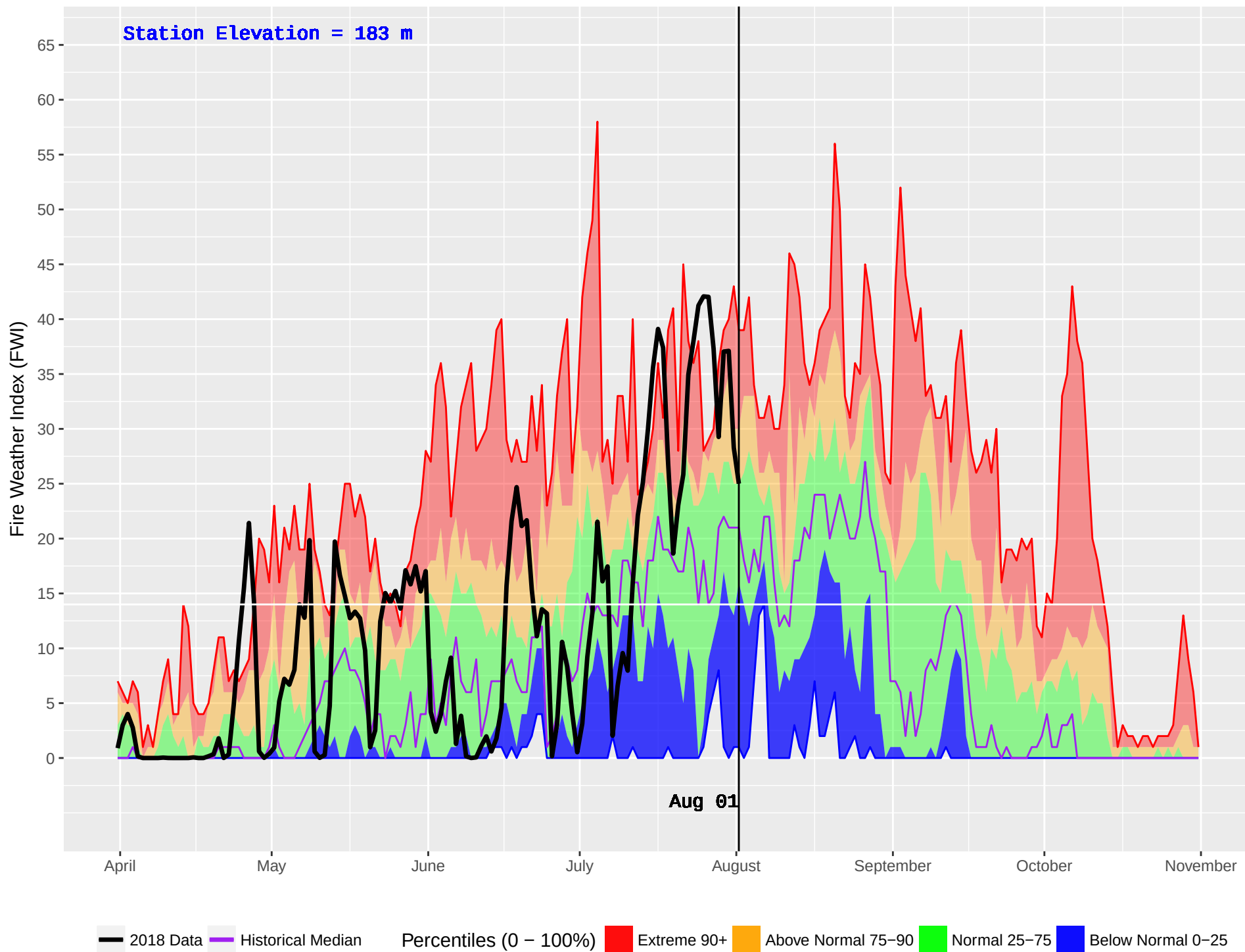
MESACHIE 2 (934) : Historical (2006–2016) and Current (2018) Daily Fire Weather Index (FWI)
